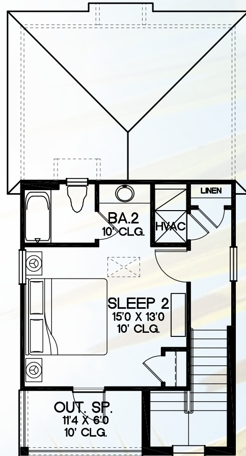
2ND FLOOR
