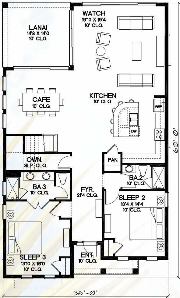
1ST FLOOR
