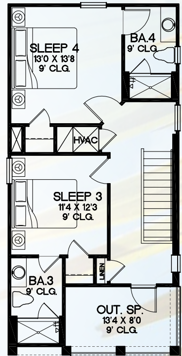
3RD FLOOR
